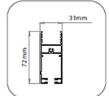
7- Frame Top Bottom Profile
