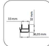
5- Frame Vertical Profile
