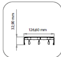
3b- 2-3 Channel Top Rail Profile
