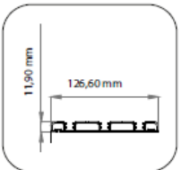
1b- 2-3 Channel Bottom Rail Profile
