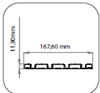
1a- 4 Channel Bottom Rail Profile
