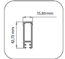
Adaptor Profile (Double Side System)
