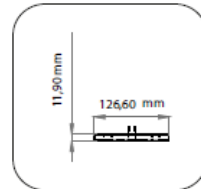
4c- 2 Channel Side Rail Profile
