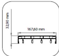
3a- 4 Channel Top Rail Profile
