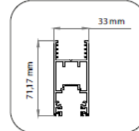
6- Frame Vertical End Profile
