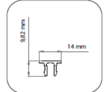
8- Bottom Rail Cover Profile
